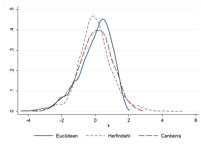
Figure C1: Kernel Density of Standardized Cultural Similarity Indexes
