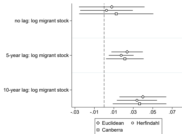
Figure C2: Baseline Regression with different lags of migration
